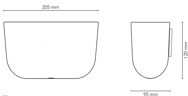
Hanger
