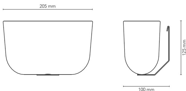
Hanger
