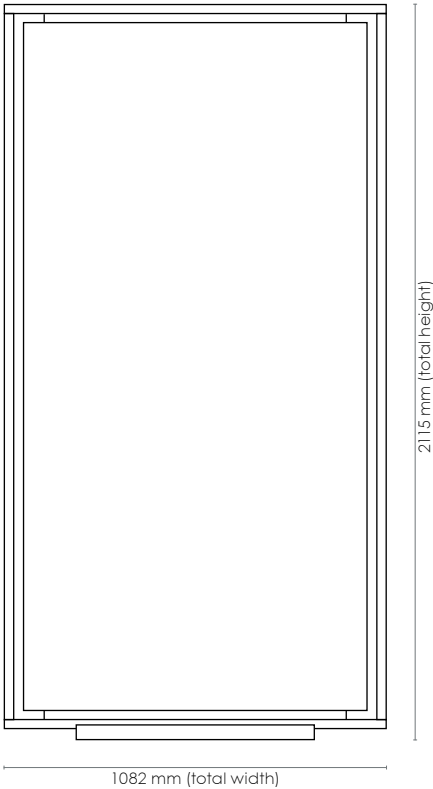
Dynamic Flex Floor stand w. Dynamic Flex Wall frame size 1082 mm x 2082 mm & board size 1000 mm x 2000 mm
